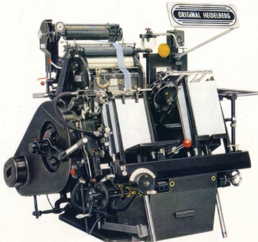
Foil stamping device of TP I
